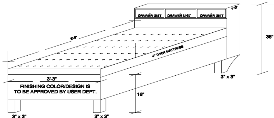
PRELIMINARY LAYOUT OF PROPOSED CUSTOMIZED BEDS & MATTRESSES AT SBILD , SALT LAKE
